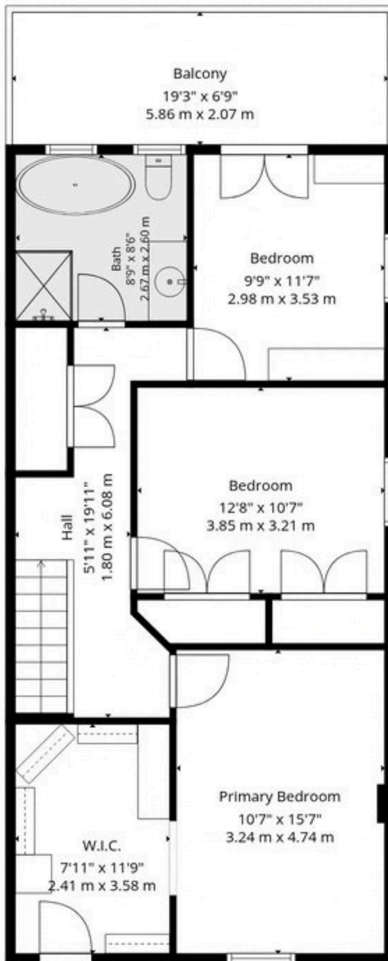
2ND FLOOR
